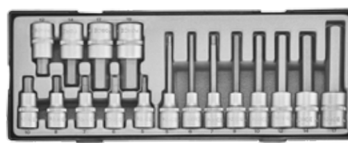
Module 17 inbus doppen 1/2" Module de 17 douilles hex 6 pans 1/2" 5-6-7-8-10-12mm (65mmL) 14-17-19 (70mmL) 5-6-7-8-10-12-14mm (100mmL) 17mm (110mmL)
